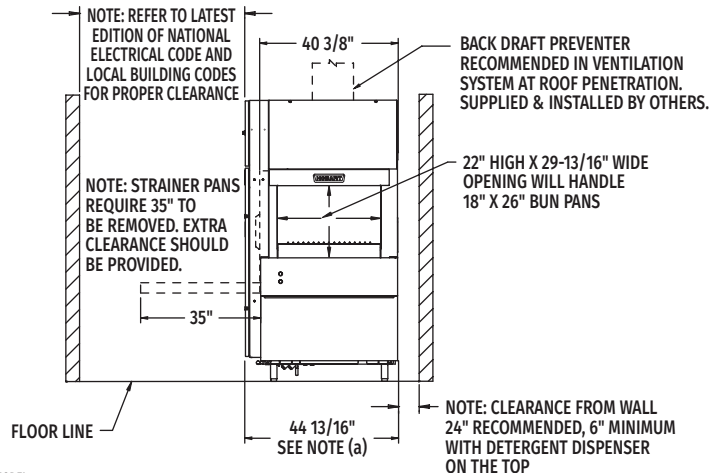
Back/Unload End
