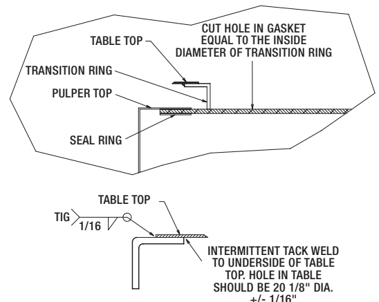
DETAIL "A" - TRANSITION RING ATTACHMENT TO TABLE BY APPLICABLE CONTRACTOR
