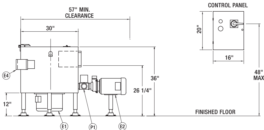
WPR-1260 ELEVATION VIEW (FREESTANDING)
